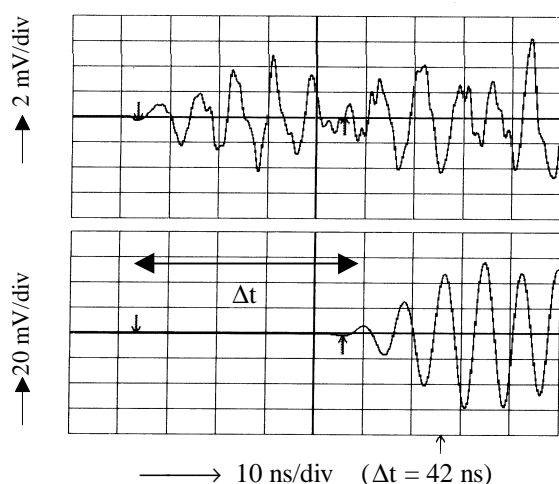
Fig. 12: Simulation of PD source localization: Waveforms
