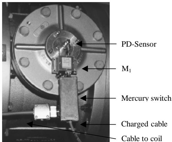
Fig. 2: Mercury switch with matching unit connected to a PD sensor
