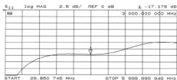
Fig. 6: Source reflection of the mercury switch
