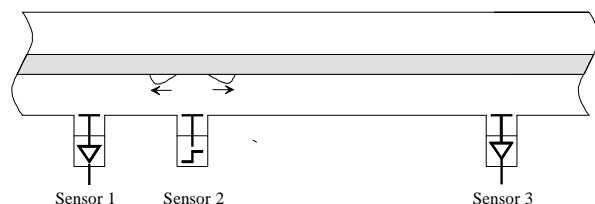
Fig. 11: Measurement setup for simulation of localization measurement. PD like pulses injected in sensor 2 and registered at sensors 1 and 3
