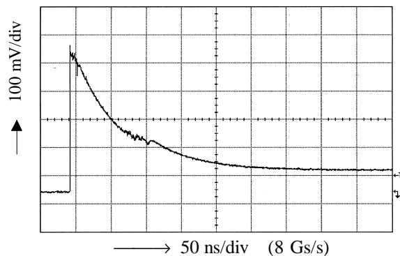
Fig. 5: Pulse shape with a charging cable of 1 meter.
