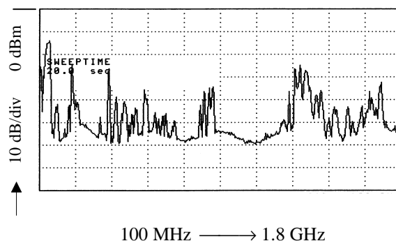
Fig. 9: Injection of pulse in a PD sensor: measured spectrum at the adjacent sensor
