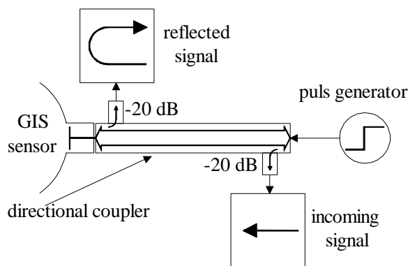
Fig. 7: Measurement setup for the determination of the pulse reflection at the sensor
