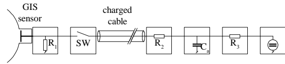
Fig. 3: Pulse generator circuit
