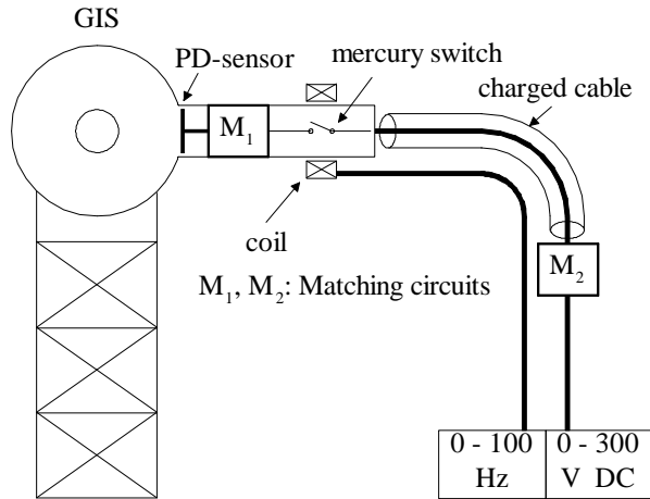
Fig. 1: Design of the pulse generator
