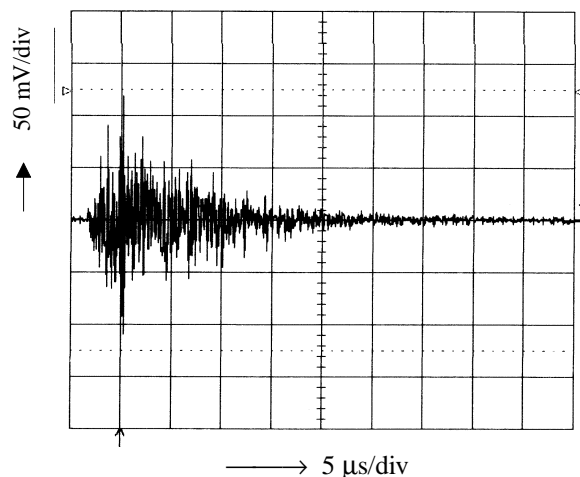
Fig.10: Sensitivity check of PD detection in GIS
