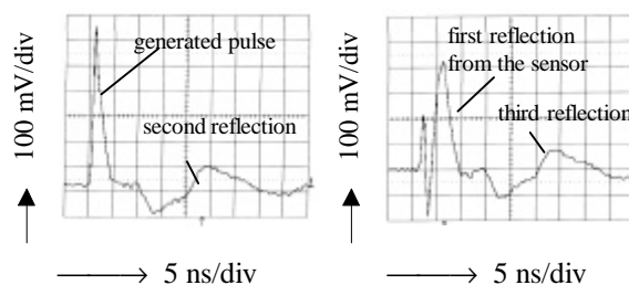
Fig. 8: Measured pulse forms of the incoming and the reflected signal (Fig. 7)
