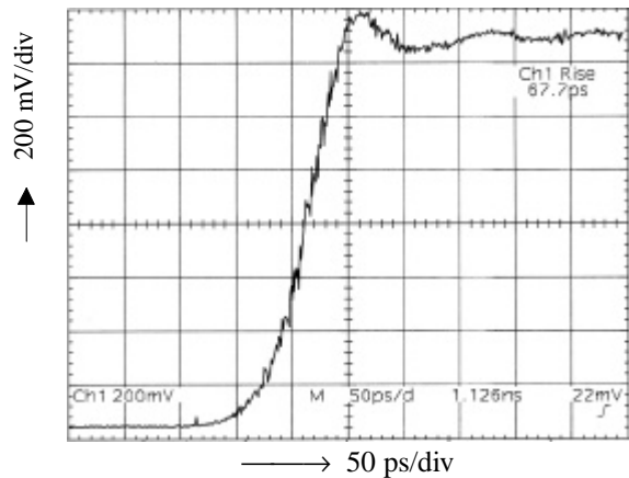
Fig. 4: Measured rise time of pulse generator
